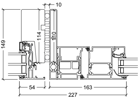
VELFAC 200 ENERGY - VELFAC 500 Outward opening door
