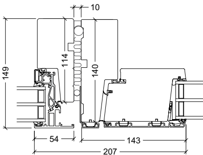
VELFAC 200 ENERGY - VELFAC Ribo Outward opening door Must be fitted with a coupling profile.
