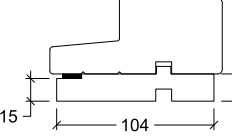
Packer type 300-128
