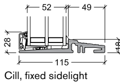
Cill, fixed sidelight
