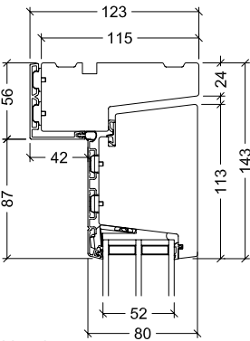
Head
