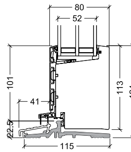
22.5mm HELO® threshold
