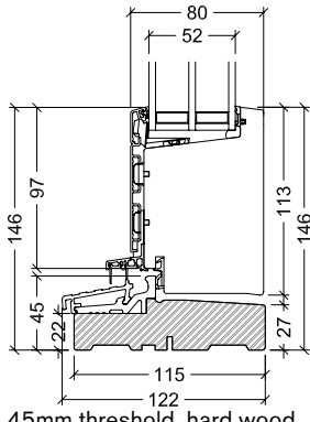
45mm threshold, hard wood
