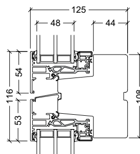
90mm transom
