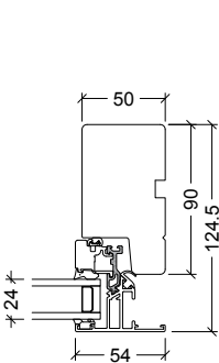
90mm frame
