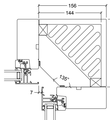
90° corner post with backboard, type A2014
