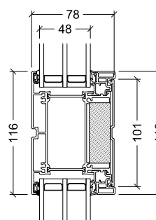
116mm glazing bar 48mm glazing
