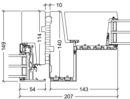
VELFAC 200 ENERGY - VELFAC Ribo Inward opening door Must be fitted with a coupling profile.
