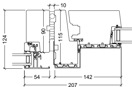
VELFAC 200 - VELFAC Ribo Inward opening door Must be fitted with a coupling profile.
