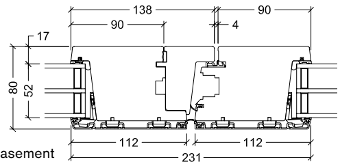
Mullion, French casement
