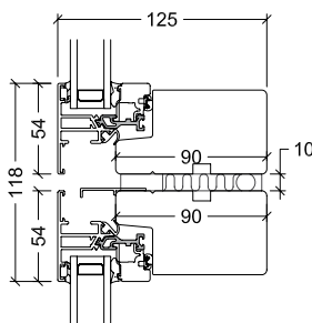
VELFAC 200 - VELFAC 200 Vertical coupling
