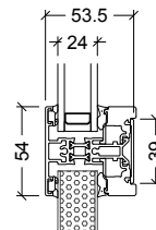
54mm glazing bar 24mm glazing
