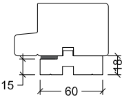
Packer type 100-886 Also available for sliding casement doors
