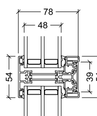
54mm glazing bar 48mm glazing
