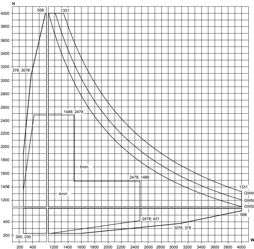
Min./max. sizes, 48mm glazing
