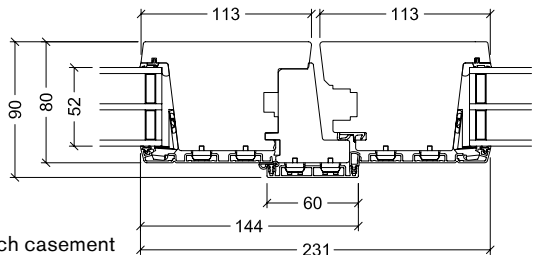
Mullion, French casement
