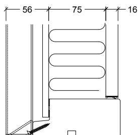
VELFAC 280 rainscreen mounted on frame from factory
