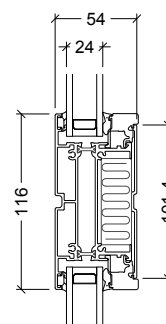
116mm glazing bar 24mm glazing
