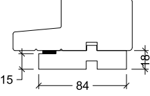
Packer type 300-130 Also available for sliding casement doors
