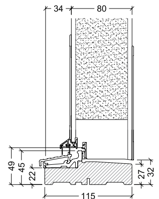
45mm threshold, hard wood
